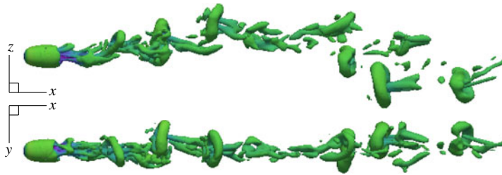
FIGURE 17. Wake observed in mode III ( Re = 1200 , m^* = 80 , l^* = 10 and U^* = 30 ) visualized with isosurface of Q = 0.001 . Flow from left to right.
