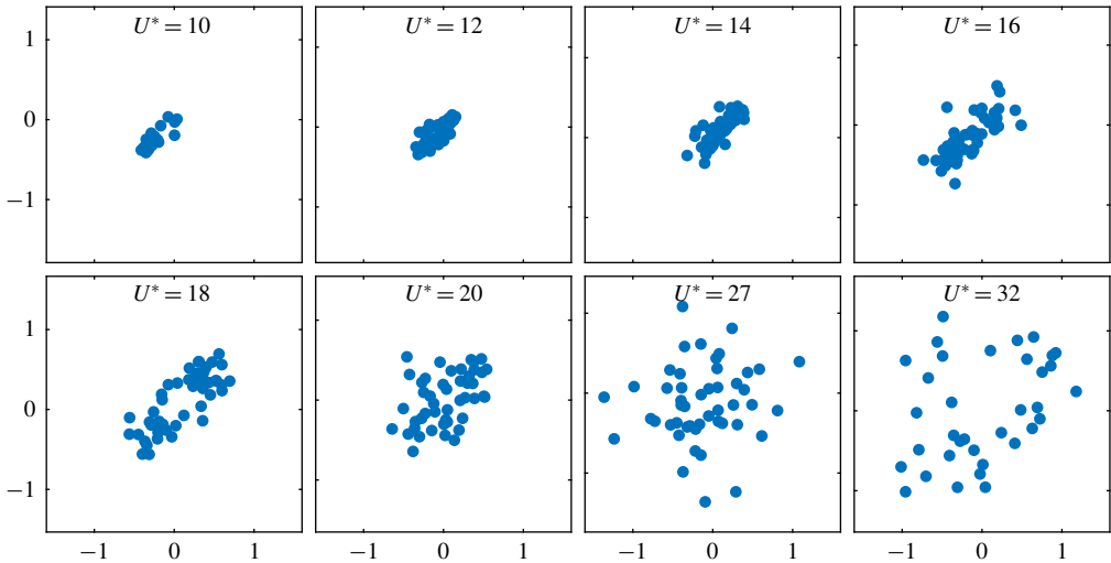
FIGURE 27. Poincaré maps for Z/D , taken from each upward zero crossing of the sphere transverse displacement for various reduced velocities: U^* = 10, 12, 14, 16, 18, 20, 27 and 32 , at Re = 1200 and m^* = 0.8 .
