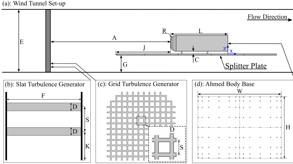
FIGURE 1. Experimental set-up (not to scale) showing: (a) schematic of wind tunnel with Ahmed body located on the splitter plane, (b) slat turbulence generator dimensions; (c) grid turbulence generator dimensions, and, (d) distribution of pressure measurement points on Ahmed body base.
