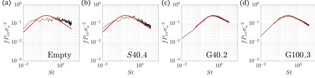
FIGURE 3. Illustration of turbulence length-scale calculation in the longitudinal direction based on von Kármán fitting (black axes) for configurations: (a) empty/no turbulence device, (b) 40 mm slats at 4 metres, (c) 40 mm grids at 2 metres, (d) 100 mm grids at 3 metres.
