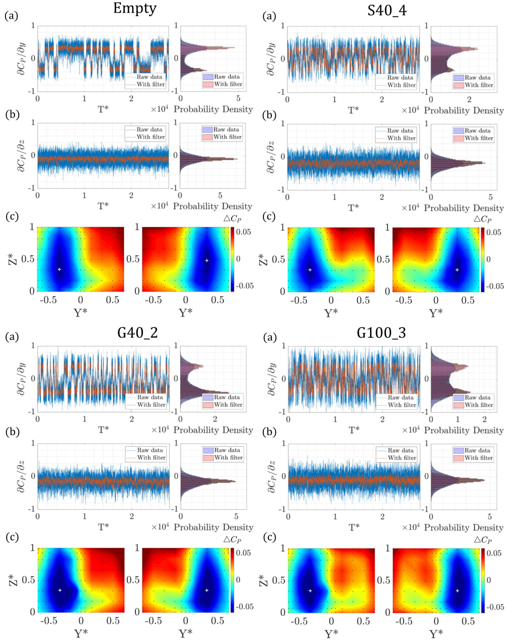
FIGURE 4. Comparison of the bistability characteristics between the Empty , S40.4 , G40.2 and G100.3 cases: (a) lateral bistability quantified by \partial C_P / \partial y signal and corresponding probability distribution; (b) vertical bistability quantified by \partial C_P / \partial z signal and corresponding probability distribution; (c) phase averaged relative pressure coefficient ( \Delta C_P = C_P - \bar{C}_P ) illustrating the bistability at left and right state, white cross shows location of minimum pressures.
