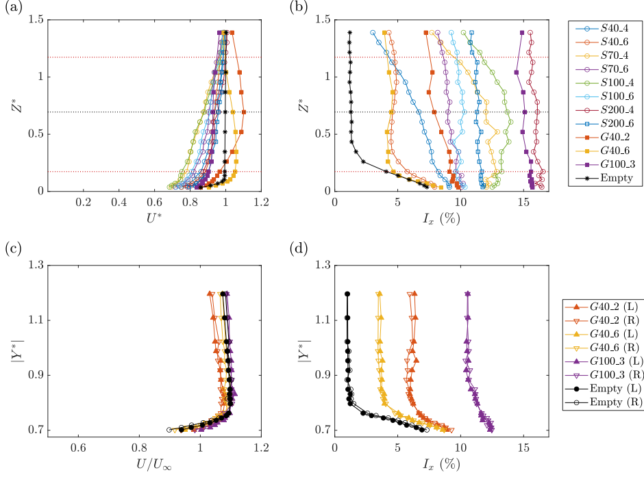
FIGURE 2. Ground boundary layer profiles at X^* = -3.625 of the Ahmed body without the presence of the Ahmed body model, (a) velocity normalised by the free stream velocity at Z^* = 1.74 ; (b) Turbulence intensity ( I_x ). Left and right Ahmed body side-surface boundary-layer profiles at mid-height upstream of separation ( X^* = -0.05 , Z^* = 1.74 ) for: (c) velocity; (d) turbulence intensity; for the empty and grid-generated turbulence cases.
