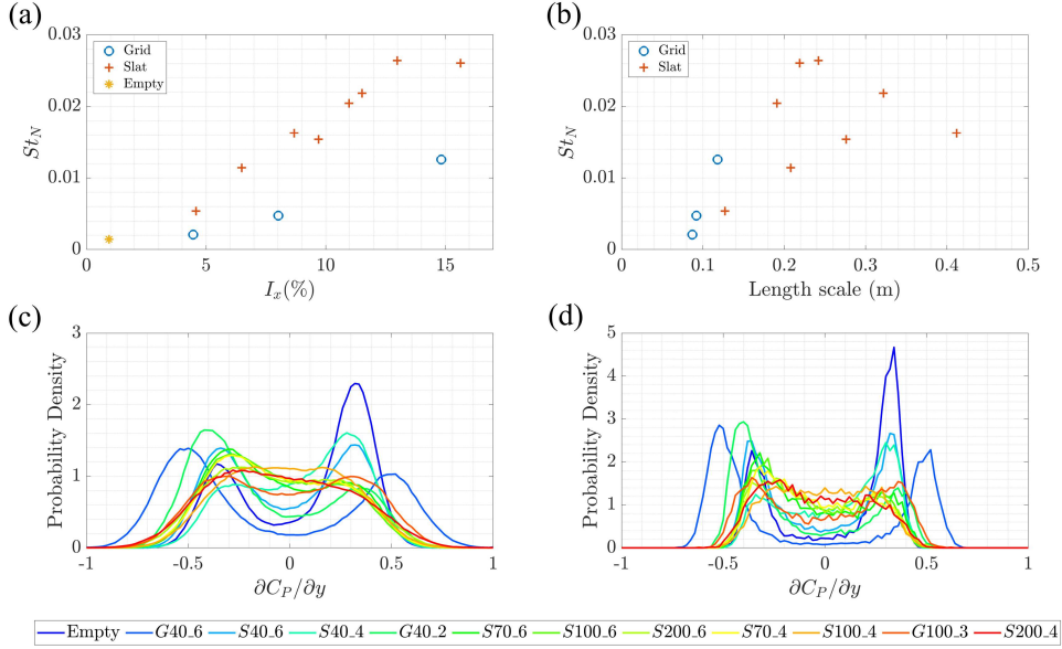
FIGURE 5. Correlation between bistability switching frequency ( St ) and: (a) turbulence intensity; (b) turbulence length scale; and probability density profiles of lateral pressure gradient without (c); and with (d) filter.
