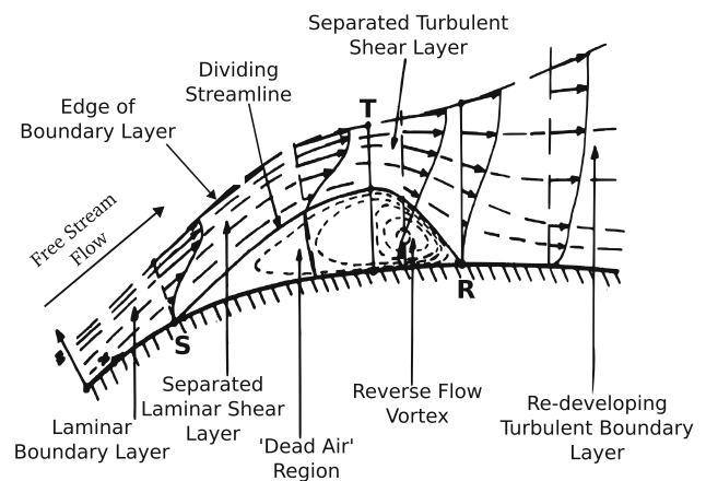
Fig. 12 Time-averaged flow features of a laminar separation bubble on the suction side of an airfoil. S: separation point, R: reattachment point, T: maximum vertical displacement where transition is most likely (Horton 1968)
