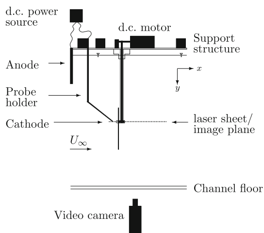
Fig. 1 Side view of the experimental set-up of the hydrogen bubble (H 2 ) rig used in flow visualisations. A single blade is aligned with the tower section in the phase-locked visualisations. Freestream flow, U_\infty is from left to right aligned with the positive x -axis. The x -, y - and z -axis follow a right-handed coordinate system. Channel depth reduced in figure. Images were captured in the x - z plane
