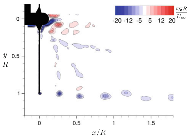
Fig. 7 Phase-locked average wake of the Tjæreborg wind turbine operating in a downwind configuration at the full-scale design tip speed ratio ( \lambda_d ) depicting the coherent vortical structures which dominate the near wake, contours of non-dimensional tangential vorticity, \overline{\omega_z}R/U_\infty
