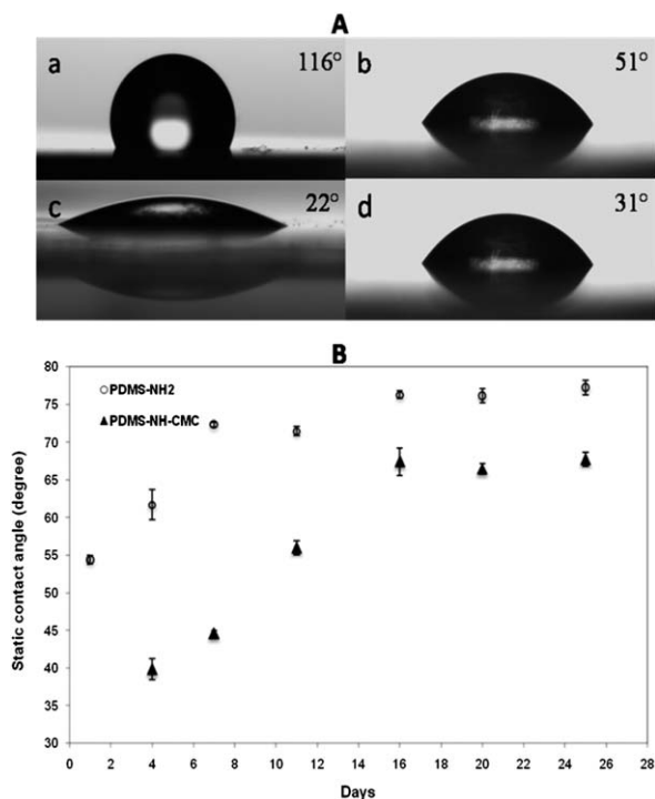
Fig. 5 (A) Static water contact angle of (a) PDMS, (b) PDMS-NH 2 , (c) PDMS-NH-CMC, and (d) PDMS-NH-CMC-GEL substrates measured at day 1. (B) shows the variation of static contact angles of PDMS-NH 2 and PDMS-NH-CMC as a function of the storage time in air.
