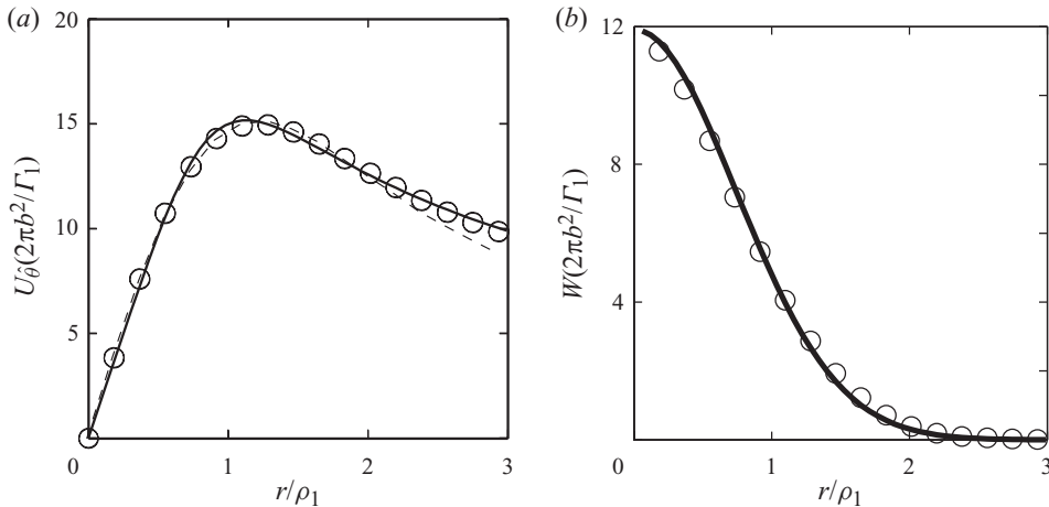
FIGURE 18. (a) Azimuthally averaged azimuthal velocity profile for the top vortex U_{\theta 1} , as a function of the radius r . The experimental points are symbolised by dots. The solid line corresponds to the VM2 model. The fit to a Gaussian model is shown by the dashed line. (b) Same as (a) for the axial velocity defect W_1 fitted to a Gaussian function.
