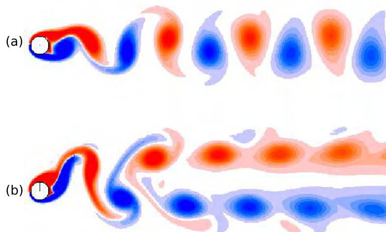
Fig. 11: The cylinder wake depicted by vorticity contours (scale -2 to 2), representative of: (a) the initial branch, U_r = 3 ; (b) the lower-type branch, U_r = 4.5 ; The damping coefficient \zeta = 0.001 .
