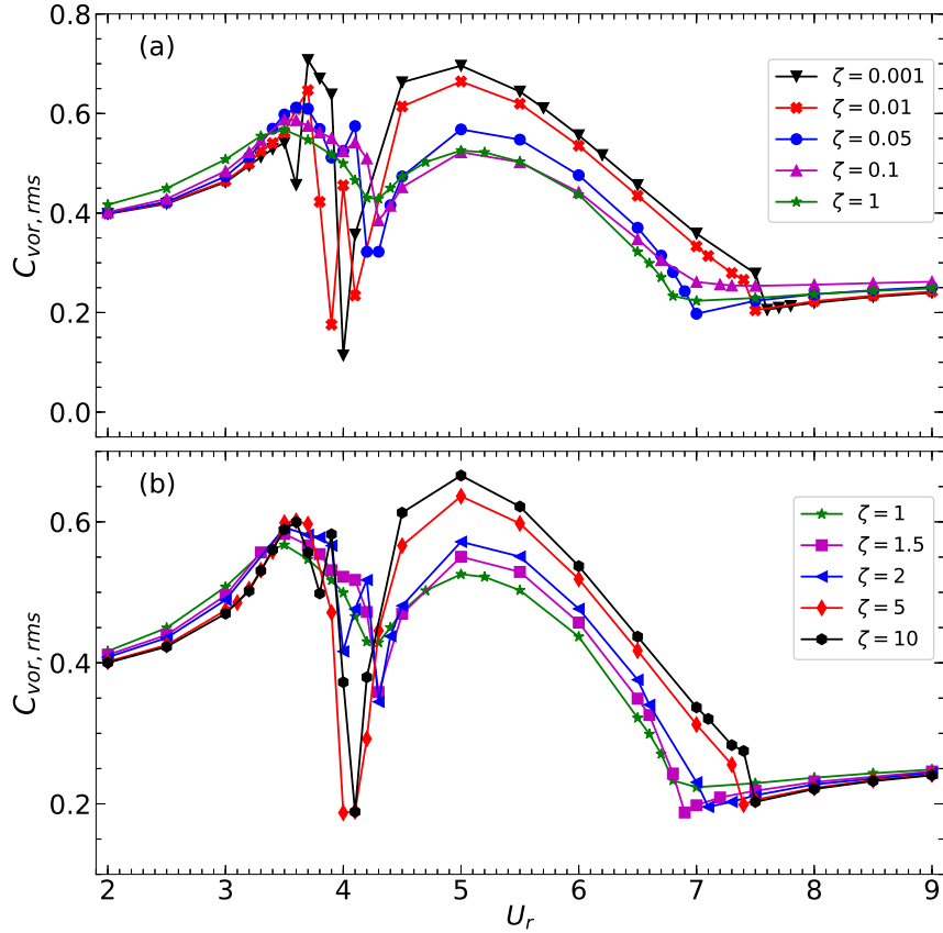
Fig. 22: Response for the mounted cylinder by comparing the RMS of the vortex force ( C_{vor} ) with reduced velocity, for damping ratio \zeta = [0.001 - 10] and R = 1 .
