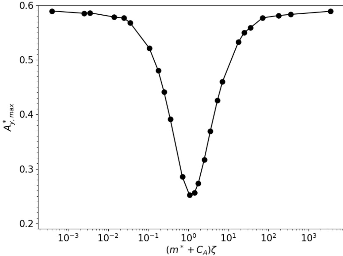
1882 Fig. 25: Griffin plot of the peak amplitude data against logarithm of the mass-damping parameter, (m^* + C_A)\zeta 1883 for R = 1 . 1884 1885
