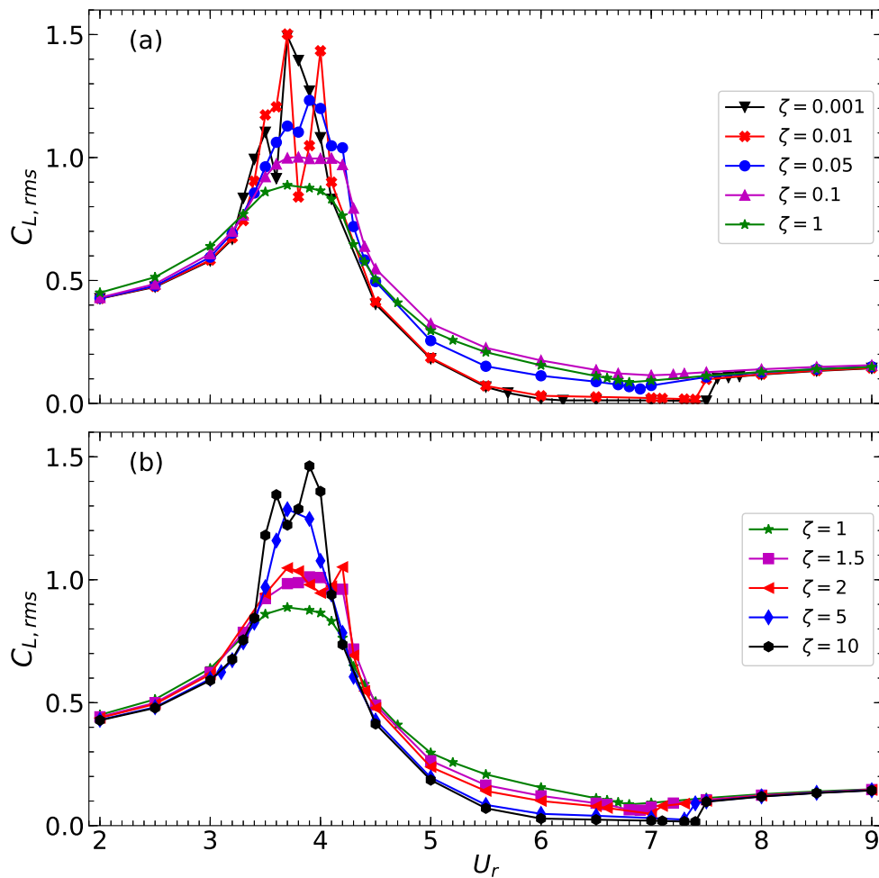
Fig. 21: Response of the mounted cylinder in term of RMS of lift force ( C_L ) versus reduced velocity, for damping ratios in the range \zeta = [0.001, 10] . Here, R = 1 .
