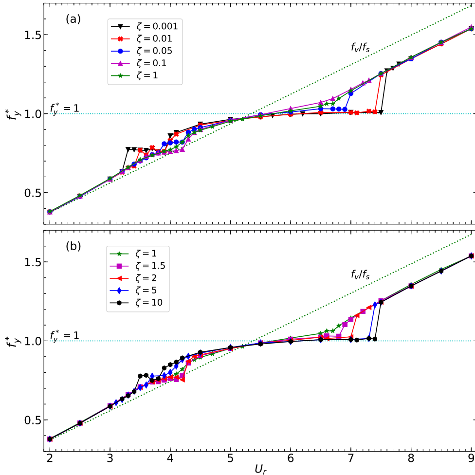
1560 Fig. 20: Comparison of normalized frequency, f^* = f_y/f_s , with various damping ratio. The green dotted 1561 line represent the vortex-shedding frequency for the stationary cylinder. 1562 1563 1564 1565 1566 1567 1568
