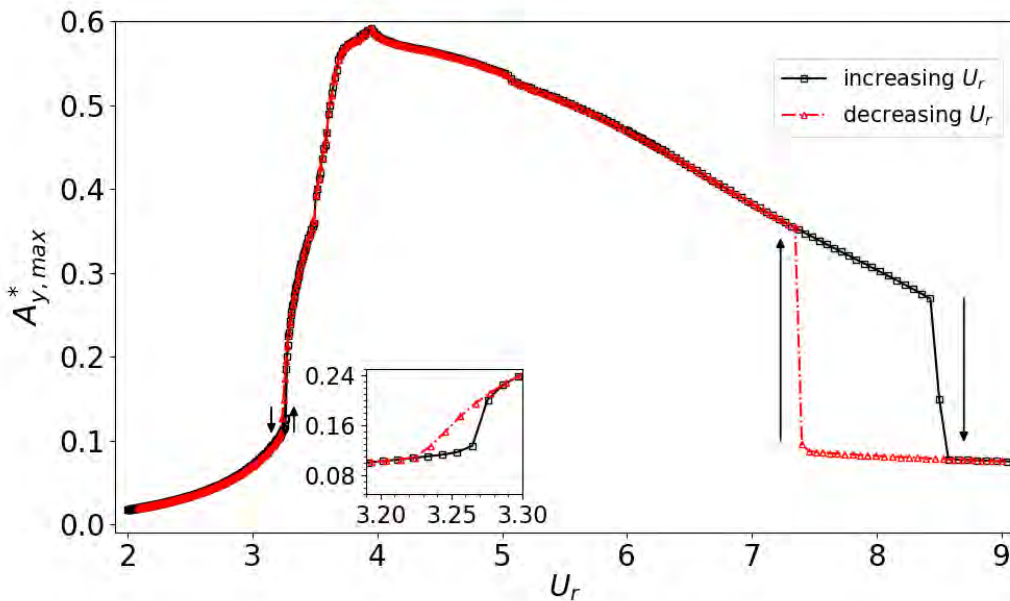
Fig. 15: Response for the cylinder mounted on a viscoelastic support. Variation of amplitude ( A_{max}^* ) versus reduced velocity ( U_r ) for \zeta = 0.001 , R = 1 using increasing and decreasing U_r .
