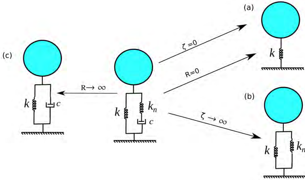
Fig. 4: Schematic of the conversion of the viscoelastic system into an elastic one: (a) R(= k_n/k) = 0 ; and (b) \zeta(= c/2\sqrt{km}) \rightarrow \infty , (c) R \rightarrow \infty . The viscoelastic (Kelvin-Voigt) model is described in (Findley and Davis (2013)).
