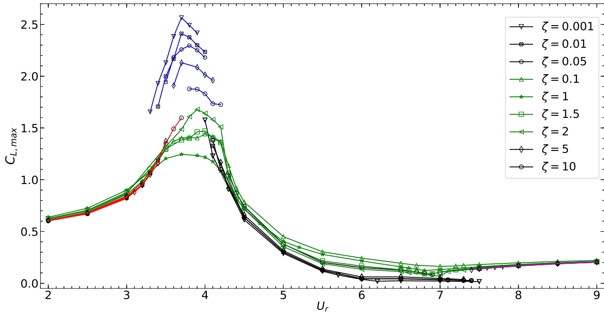
Fig. 18: Variation of maximum lift ( C_{L,max} ) versus reduced velocity ( U_r ) for damping coefficients \zeta \in [0.001, 10] .
