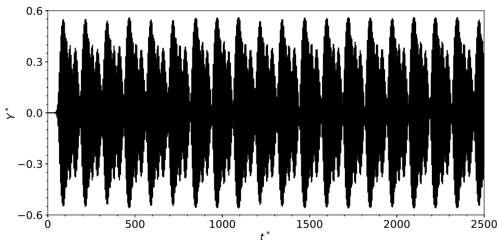
Fig. 12: The amplitude response signal for U_r = 3.7 , \zeta = 0.001 .
