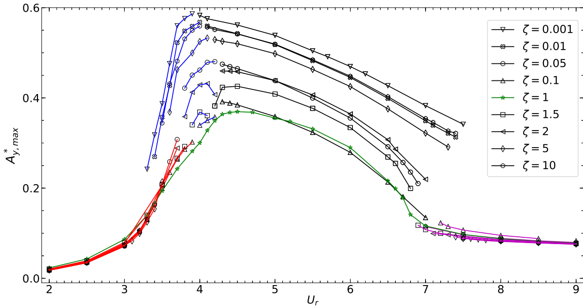
755 756 757 758 759 760 761 762 763 764 765 766 767 768 769 770 771 772 773 774 775 776 777 Fig. 6: Response for the cylinder mounted on a viscoelastic support. Variation of amplitude ( A_{y,max}^* ) versus 778 reduced velocity ( U_r ) for damping coefficient in the range \zeta \in [0.001 - 10] . The stiffness ratio ( R = 1 ) and 779 mass ratio ( m^* = 2.546 ) are fixed.
