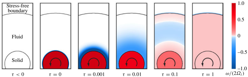
FIGURE 13. (Colour online) Evolution of the vorticity distribution for the forced cylinder case. Parameters and data are the same as in figure 12(c). (If viewing in greyscale please refer to figure 12(c) to help interpret the colourmap.)
