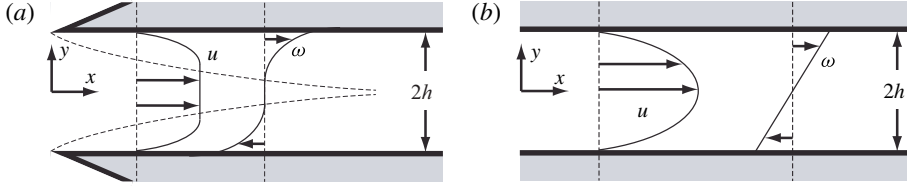
FIGURE 5. Schematic of Poiseuille flow: (a) inlet and (b) fully developed.
