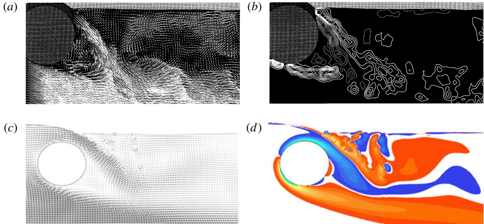
FIGURE 18. (Colour online) Flow around a submerged cylinder for Fr=0.6 . (a) Velocity and (b) vorticity fields from experiments by Sheridan et al. (1997) with G/D = 0.31 at Re = O(10^4) . (c) Velocity and (d) vorticity fields from two-dimensional simulations by Reichl et al. (2005) for G/D = 0.25 and Re = 180 . (All results reproduced with permission.)
