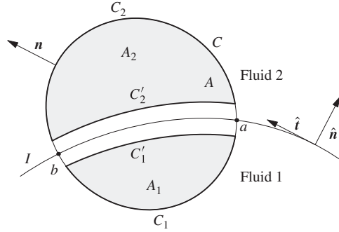
FIGURE 2. The interface I with normal vector \hat{\mathbf{n}} and tangential vector \hat{\mathbf{t}} , forming a right-handed coordinate system. Shaded subregions A_1, A_2 of the region A in each fluid are bounded by the curves C_1, C'_1 and C_2, C'_2 respectively. The outward normal vector of a region is denoted \mathbf{n} .
